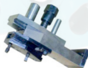
Vertical Slide with Tool Holder Rear
